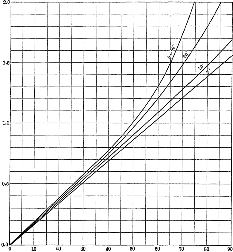
FIG. 2. The Elliptic Integral F(\theta, \phi) . k = \sin \theta . \longrightarrow \phi
